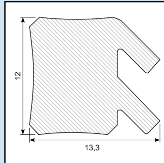
Material: CR black Hardness: SH 65
