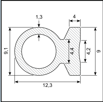
Balloon profile Hardness: SH 65
