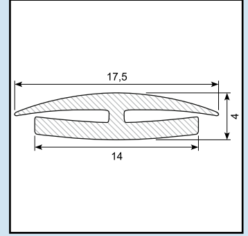
Material: EPDM black Hardness: SH 84
