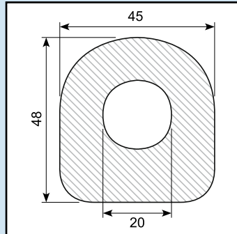
Material: NBR black Hardness: SH 60
