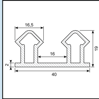
Material: Silicone grey Hardness: SH 60
