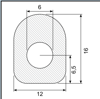
Material: NBR black Hardness: SH 65
