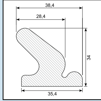
Material: EPDM black Hardness: SH 65
