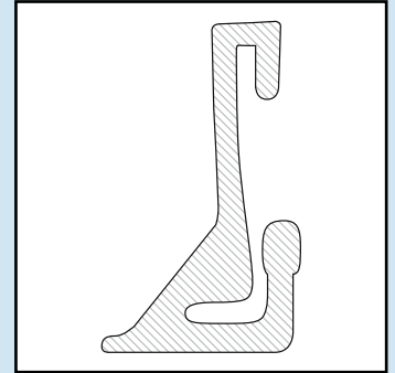
L-profile Material: EPDM Hardness: SH 70 Roll of 50 m
