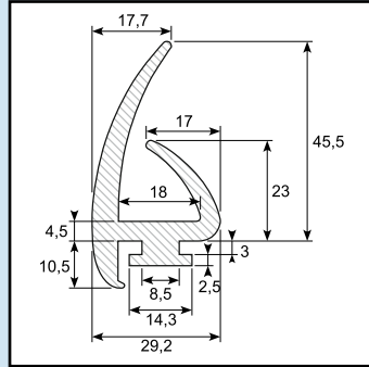
Rubber profile for alu. track Material: EPDM Hardness: SH 70
