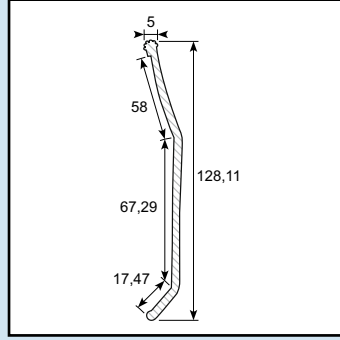
Skirt profile Material: PVC black Hardness: SH 80 Height: 125 mm Length: 1 m Roll of 64 m
