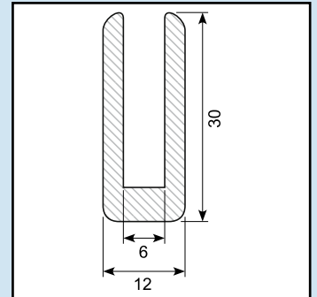
U-profile Material: EPDM Hardness: SH 70
