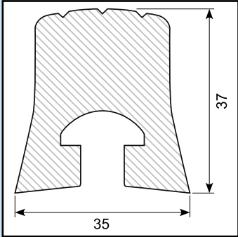
Fender profile with channel Material: PE Length: 3 m
