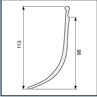
Skirt profile Material: PVC white Roll of 14 m
