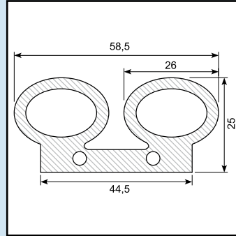
Material: Silicone blue Hardness: SH 60
