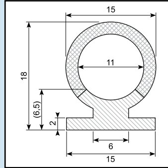
Co-ex profile Material: EPDM / sponge rubber Hardness: SH 80
