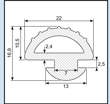
D-weatherstrip Material: EPDM Hardness: SH 70
