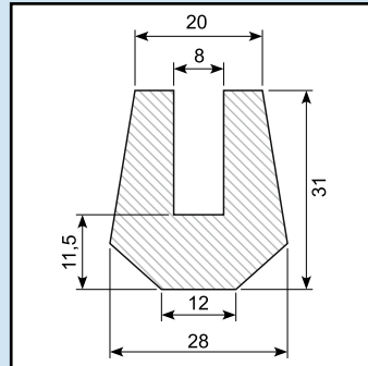
U-profile Material: EPDM Hardness: SH 70 Roll of 25 m
