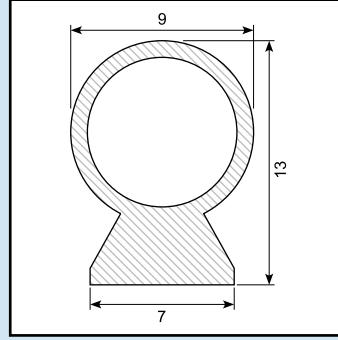
Rubber profile Material: EPDM Hardness: SH 60 / 65
