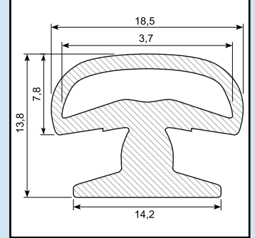
Material: EPDM black Hardness: SH 65
