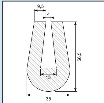
U-profile Material: EPDM Hardness: SH 65 Roll of 25 m
