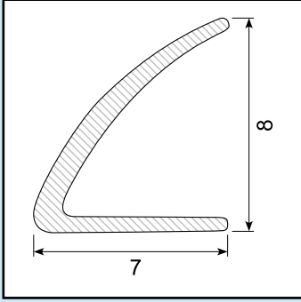
Material: Silicone white Hardness: SH 60 30.OT1024 with adhesive
