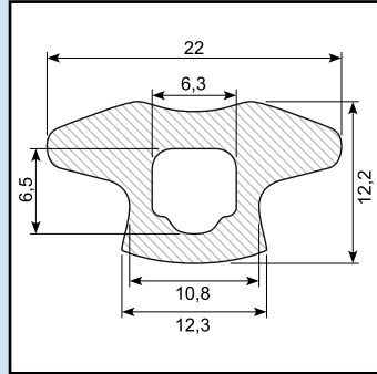
Rubber profile Material: EPDM Hardness: SH 65
