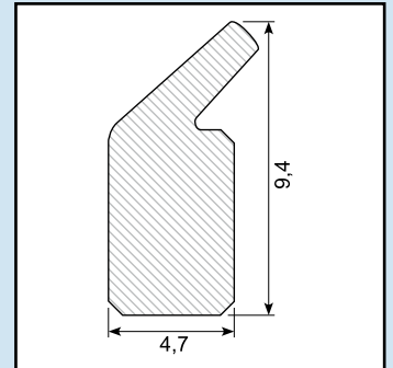
Material: CR black Hardness: SH 65
