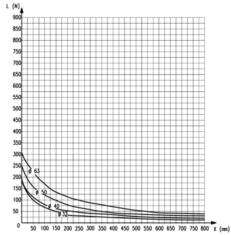
Guide "U" moving on bush (45NUT)
